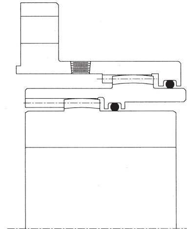
DOUBLE FLEX
