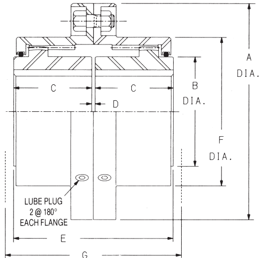
SIZE 200 THRU 207
