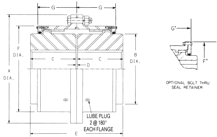
SIZE 208 THRU 230
