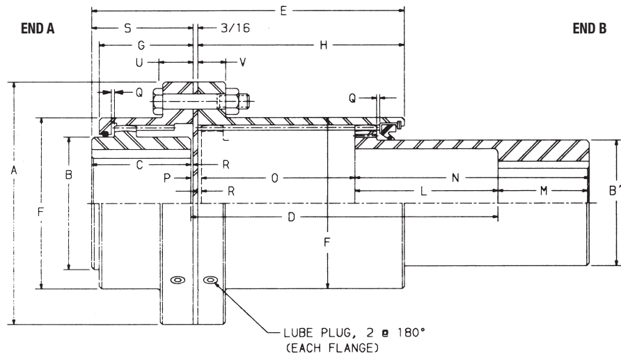
SERIES FA
