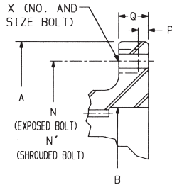
SIZES 201 1 / 2 -207
