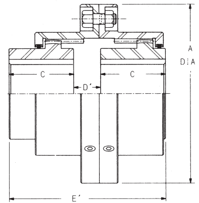
SERIES F ONE HUB REVERSED
