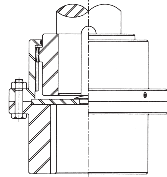
FIG. C TANDEM - VERTICAL
