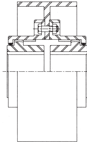
SERIES FB
