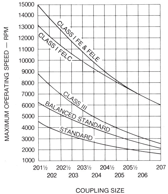
FE AND FEL AT 10-INCH SHAFT-TO-SHAFT
