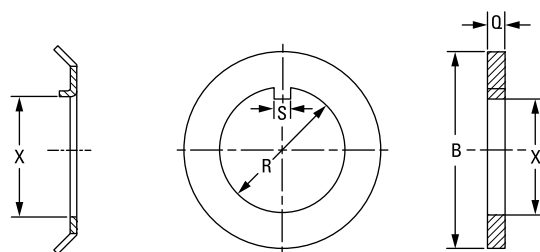
Fig. 51. Tongued washers.
