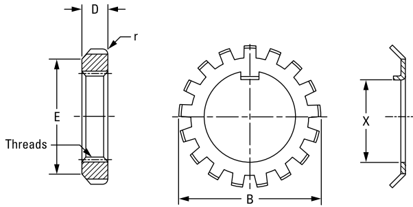
Fig. 52. Locknuts (threads are ISO 965/1, class 5H).
