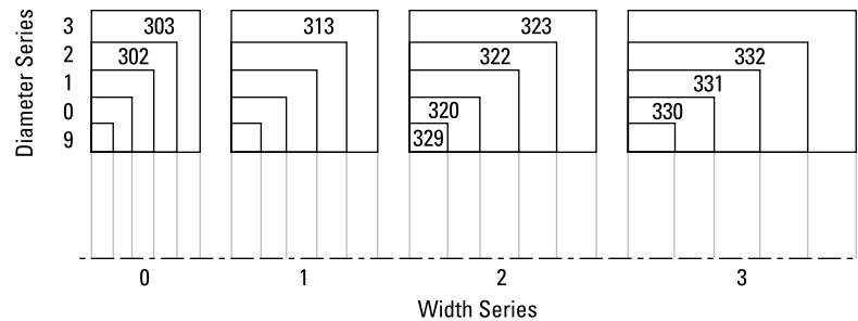
Fig. 31. Original ISO part-numbering system.
