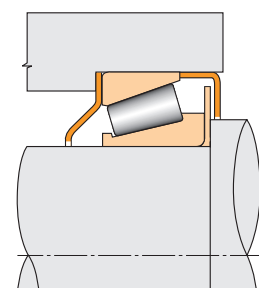
Fig. A-33 Metal stampings.
