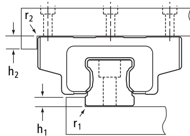
Figure 5. Shoulder Heights and Corner Radii
