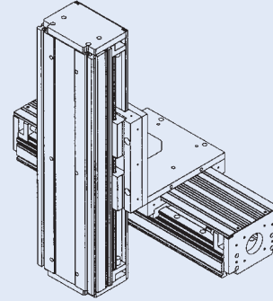
Carriage-to-Carriage XZ configuration (side mounted)
