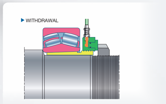
Mounting on withdrawal sleeve by indirect pushing of the hydraulic nut
