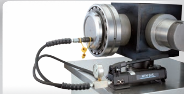
Hydraulic removal
