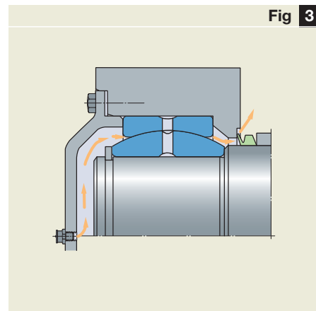
Relubricating the bearing from the side
