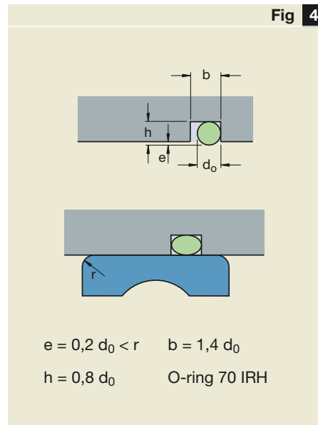
Dimensions of O-ring groove
