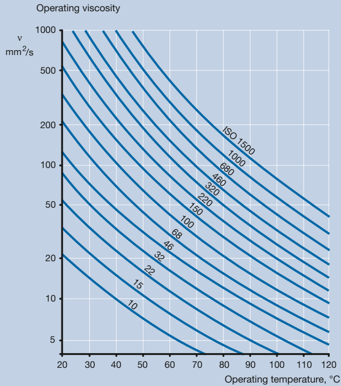
Estimation of the actual operating viscosity v
