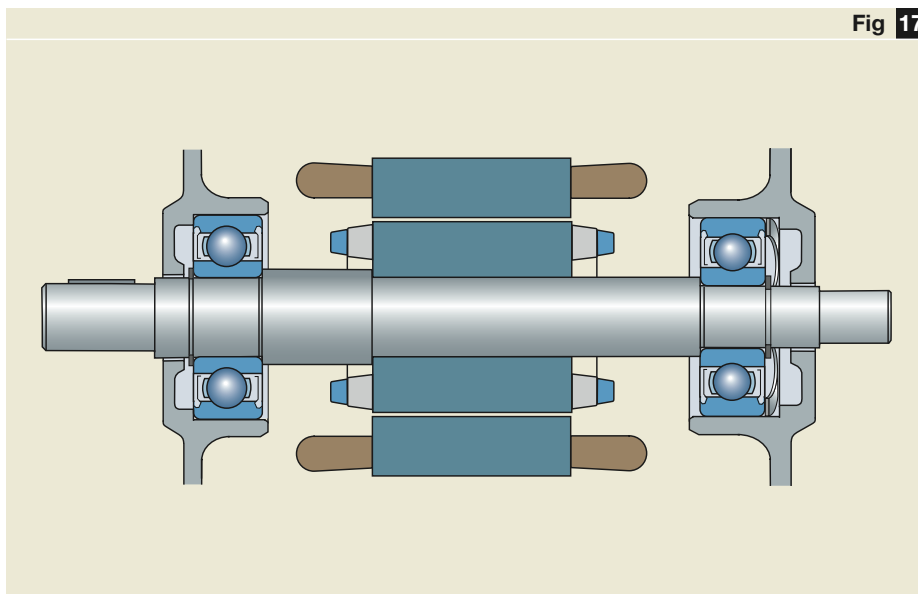
Bearing arrangement with spring preloaded deep groove ball bearings
