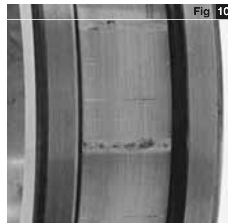
False brinelling in a cylindrical roller bearing due to vibration at standstill
