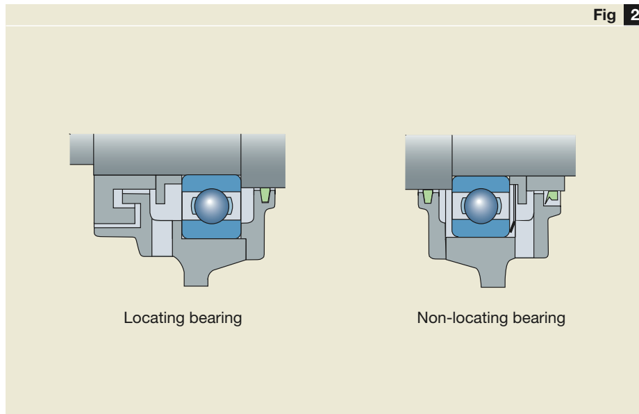
Locating and non-locating bearings
