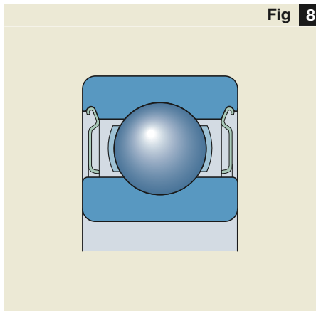
Bearing with metallic shields – 2Z
