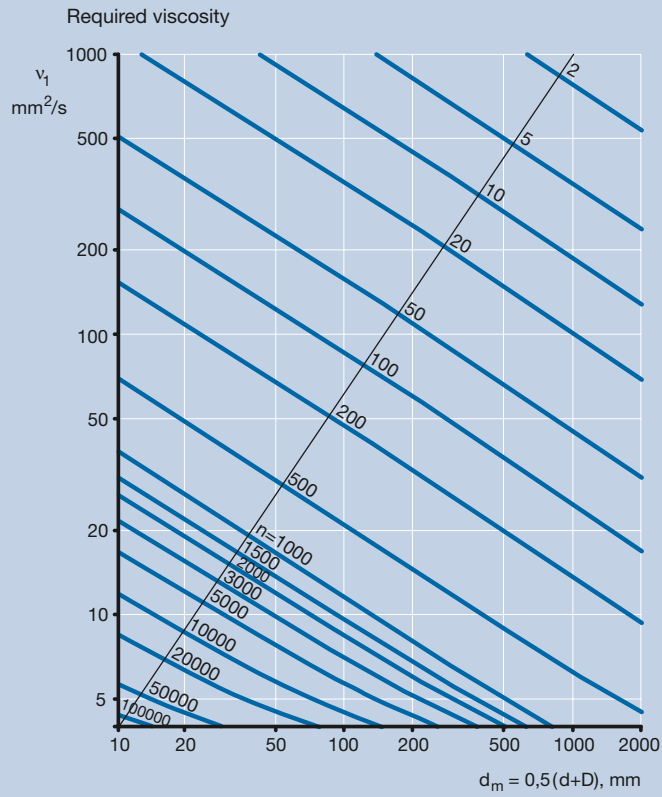
Estimation of the rated viscosity v_1 required for adequate lubrication
