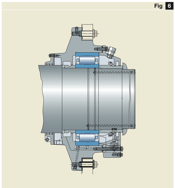
A flanged housing unit with a CARB toroidal roller bearing
