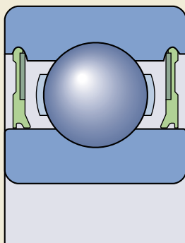
RZ seal design
