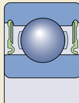
RS1 seal design
