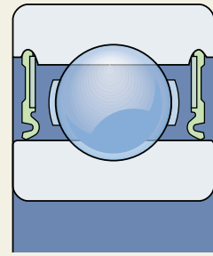
Seals of RS1 design
