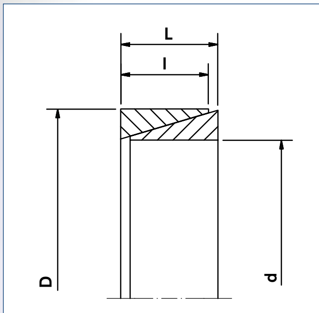
RINGFEDER® Locking Elements RfN 8006 · Dimensions
