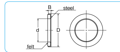
Figure C-12 Felt Seal
