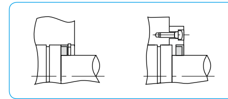
Figure C-13 Example of Felt Seal Installation
