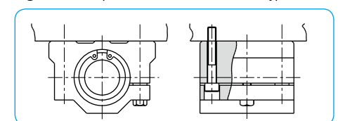
Figure C-21 Special Installation of SMJ Type
