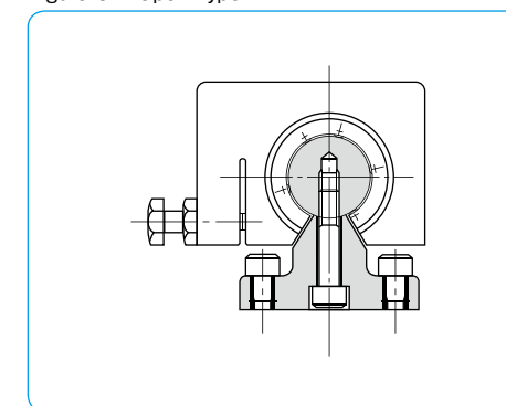
Figure C-7 Open Type
