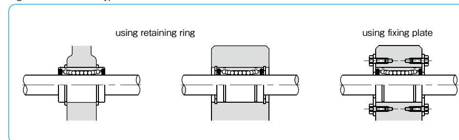
Figure C-5 Standard Type
