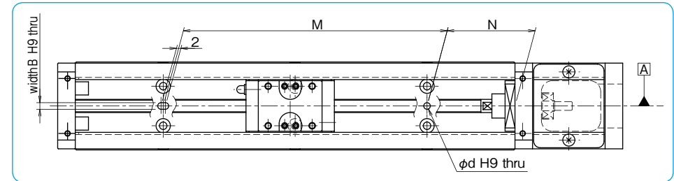
Figure H-18 Positioning Pin Hole Location
