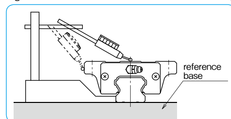
Figure A-2 Measurement Method for Motion Accuracy
