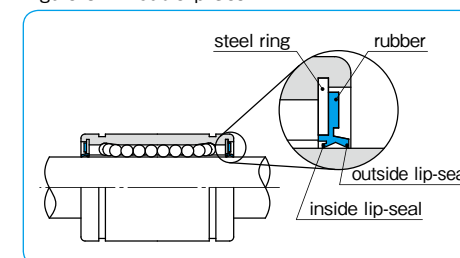
Figure C-4 Doublelip-Seal
