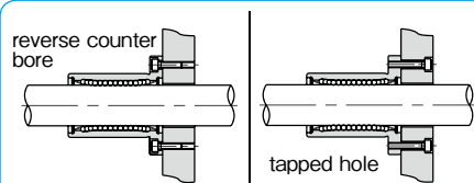
Figure C-15 Examples of Special Installation Hole
