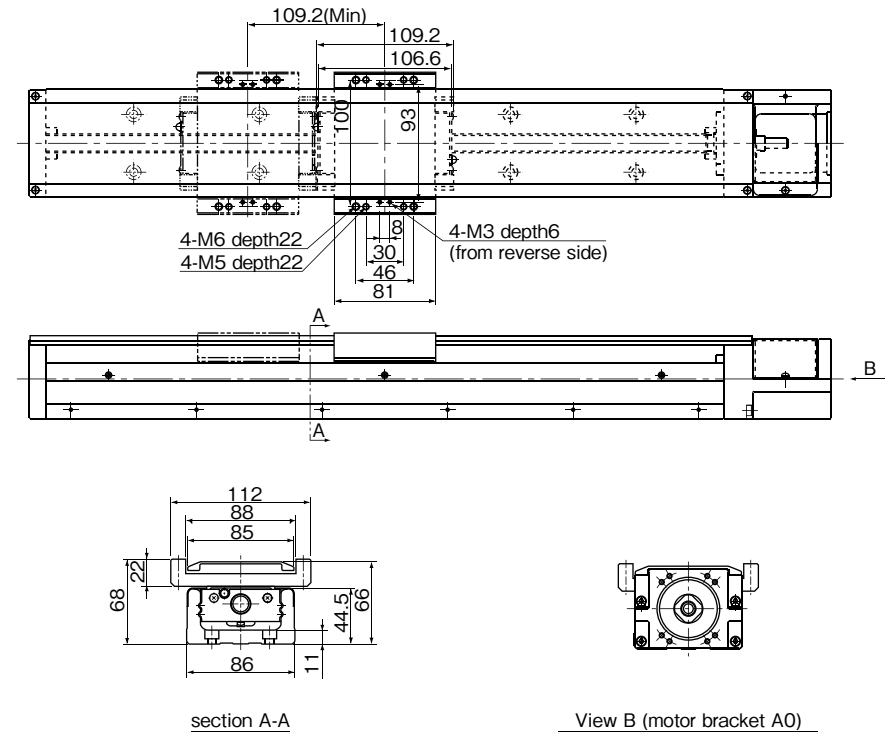
View B (motor bracket A0) refer to page H-26 for other motor bracket
