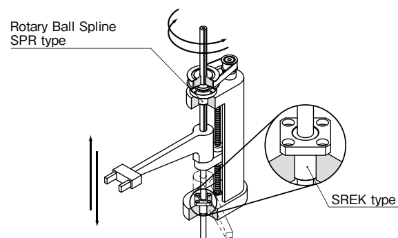
Application Example 2 Multiple Gearing Idler
