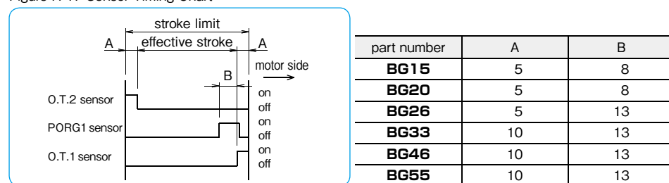
Figure H-17 Sensor Timing Chart
