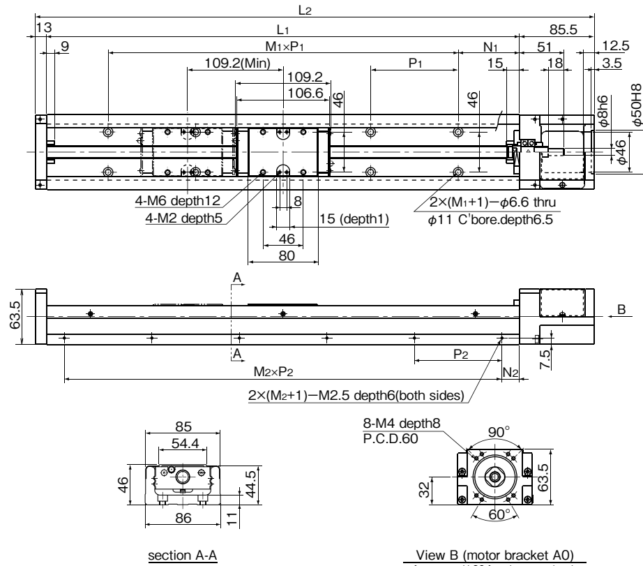
View B (motor bracket A0) refer to page H-26 for other motor bracket
