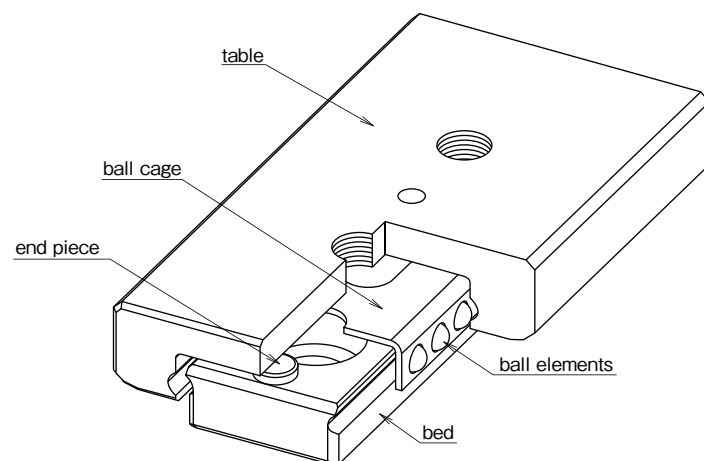
Figure G-20 Structure of SYBS type
