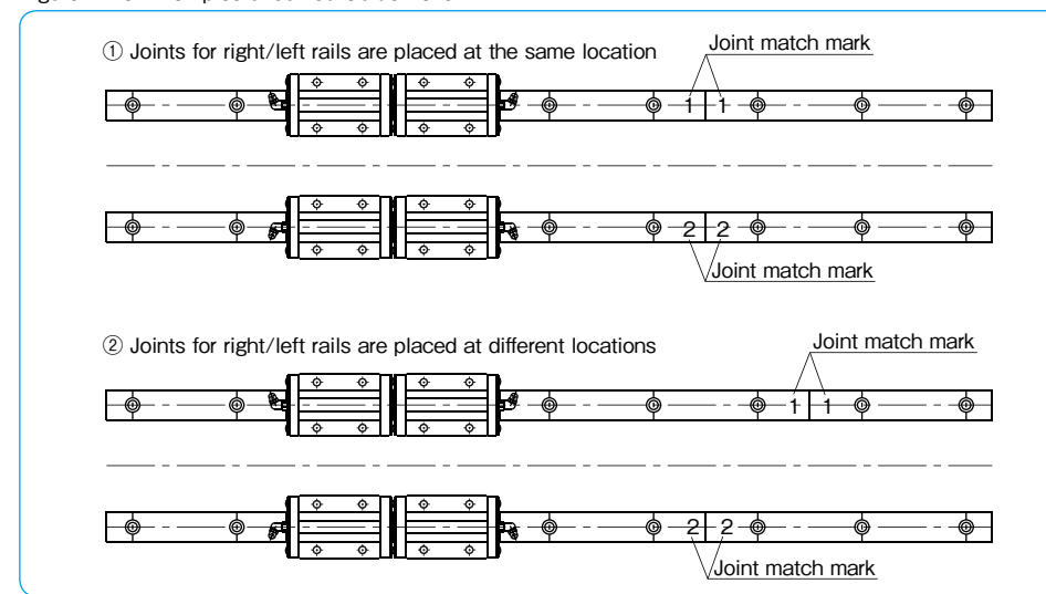
Figure A-23 Examples of Joined Guide Rails
