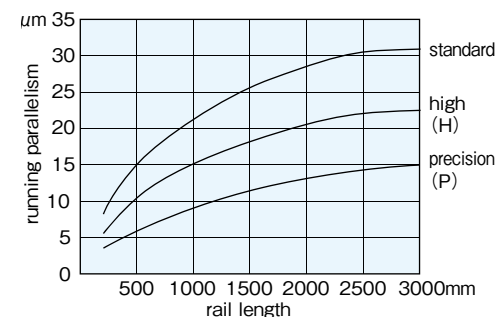
Figure A-61 Motion Accuracy
