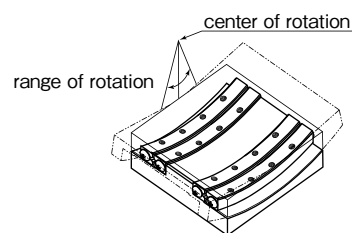
Figure G-37 Example of Installation
