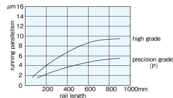
Figure A-49 Motion Accuracy
