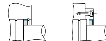
Figure E-5 Example of Installation
