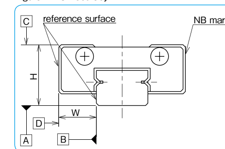
Figure A-48 Accuracy
