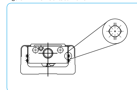
Figure H-2 Ball Contact Profile
