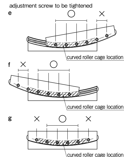
Figure G-39 Installation Method (2)
