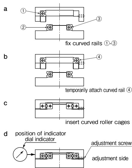
Figure G-38 Installation Method (1)
