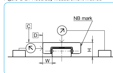
Figure G-21 Accuracy Measurement Method
