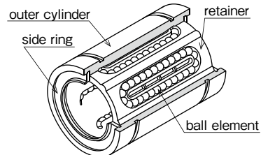
Figure C-1 Basic Structure of NB Slide Bush (SM, KB, SW)
