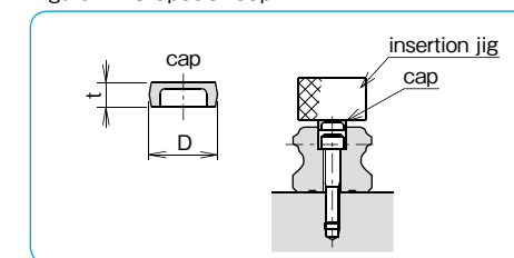
Figure A-28 Special Cap
