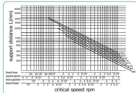
Figure I-2 Critical Speed and Support Distance
