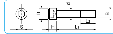
Figure G-15 Special Mounting Screw
