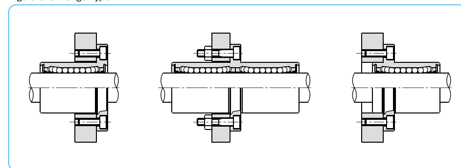
Figure C-8 Flange Type
