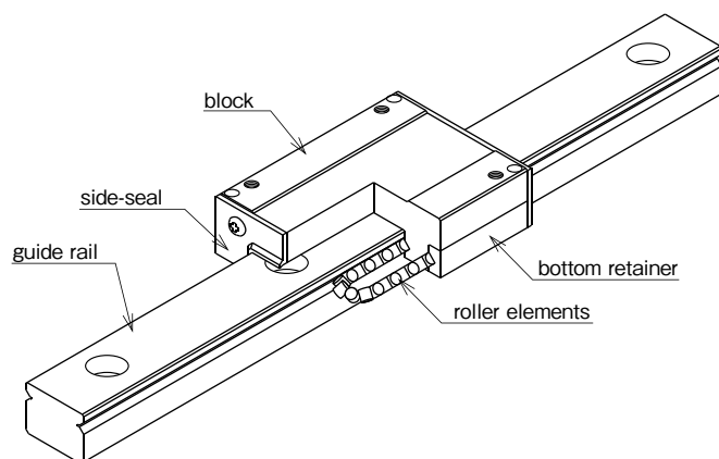
Figure A-47 Structure of SER type Slide Guide
