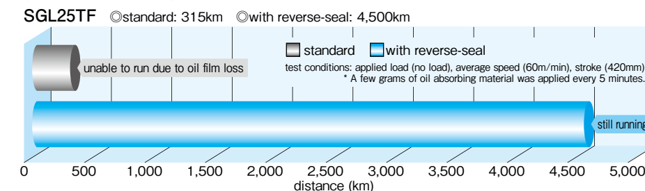
Figure A-34 Grease Dry-up Test Data
