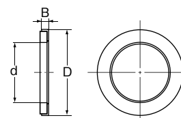
Figure E-4 Felt Seal
