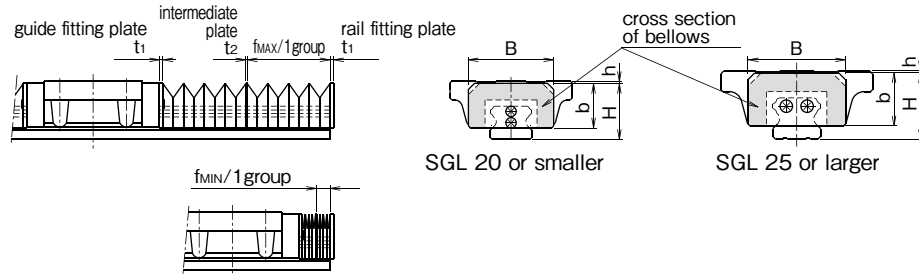
Figure A-35 Dimensions of Slide Guide with Bellows
