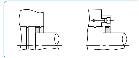
Figure C-17 Example of Felt Seal Installation
