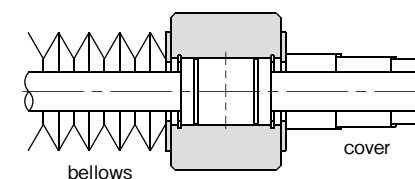
Figure 1-18 Example of Dust Prevention
