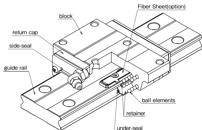
Figure A-60 Structure of SGW type Slide Guide
