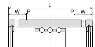
Figure E-2 Outer Cylinder Measurement Points
