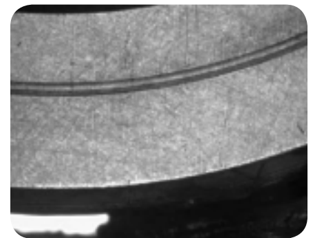
Run-in groove after 24 hours
