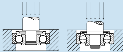
Incorrect method of fitting shaft in ball bearing without the use of a fitting aid.
