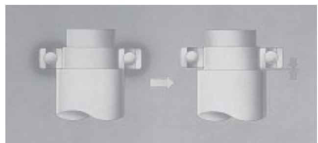
● Figure 9.3 Shaft Shoulder Gap After Cooling
