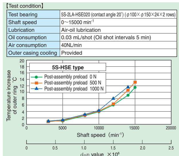
Fig. 9.24 Relationship between preload and temperature increase
