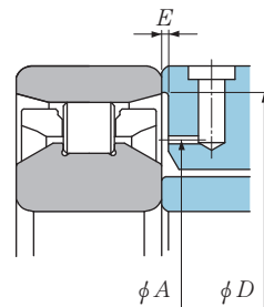
Fig. 7.8 N10HSR type
