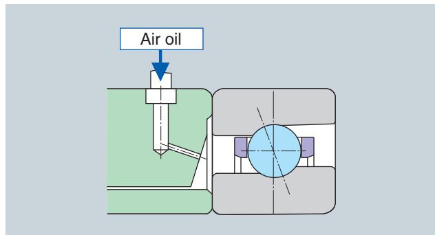
Fig. 9.23 HSE type
