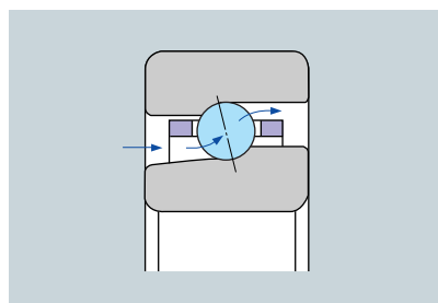
Fig. 9.4 Ultra-high-speed angular contact ball bearings
