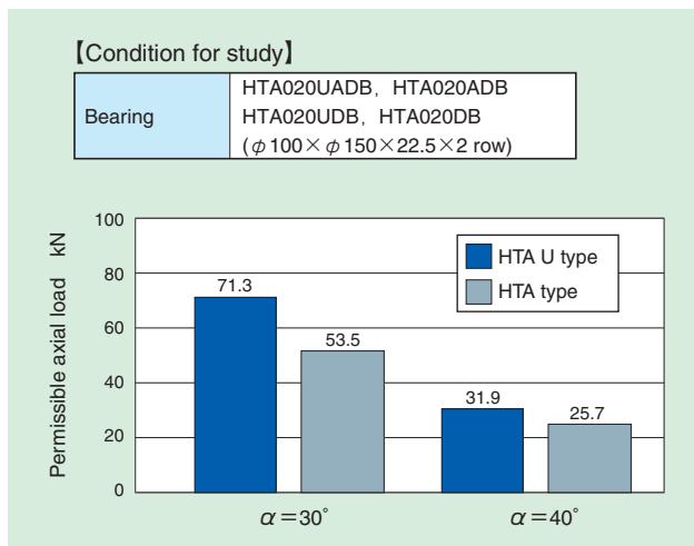
Fig. 11.4 Comparison of permissible axial load
