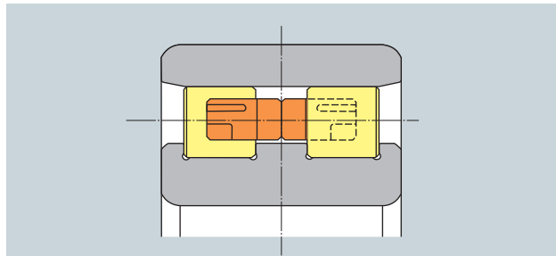
Fig. 10.4 NN30HSRT6 type
