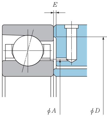
Fig. 7.5 78C, 79C, 70C and 72C types
