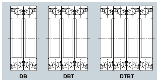
Fig. 13.2 Bearing arrangement
