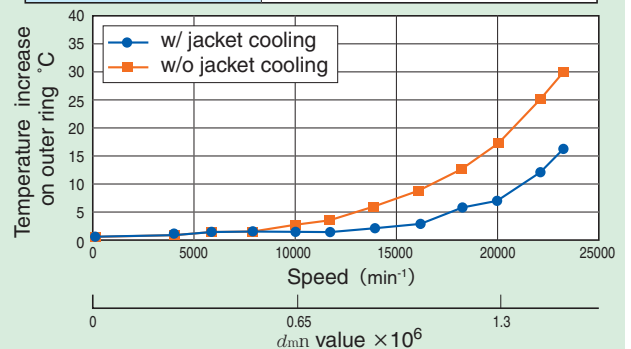
Fig. 9.22 High-speed test with air-oil lubrication
