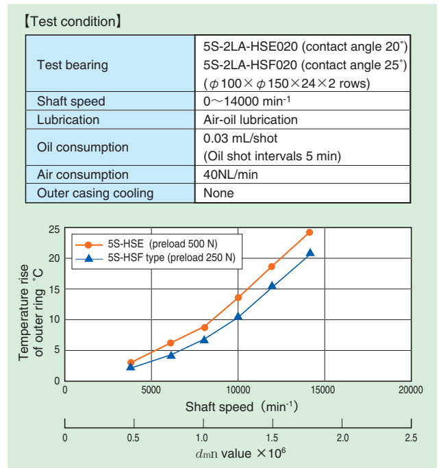
Fig. 9.27 Comparison of temperature rise
