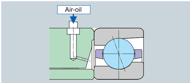
Fig. 9.20 79U and 70U types
