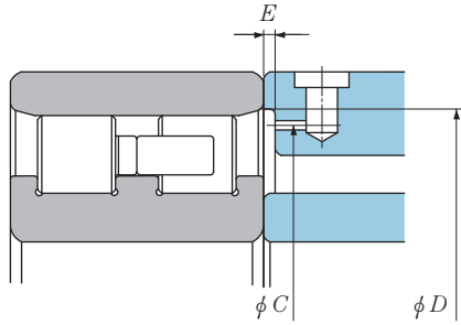
Fig. 7.6 NN30 and NN30T6 types
