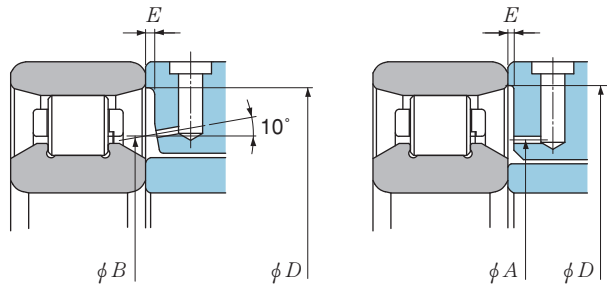
Fig. 7.7 N10HS type
