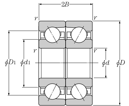
Face-to-face (DF)
