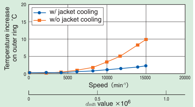
Fig. 9.21 High-speed test with grease lubrication
