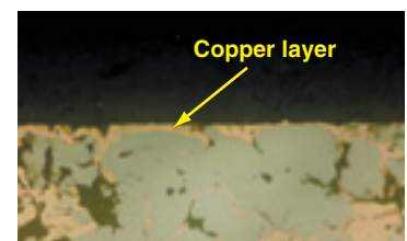
Bearing Cross Section Photograph
