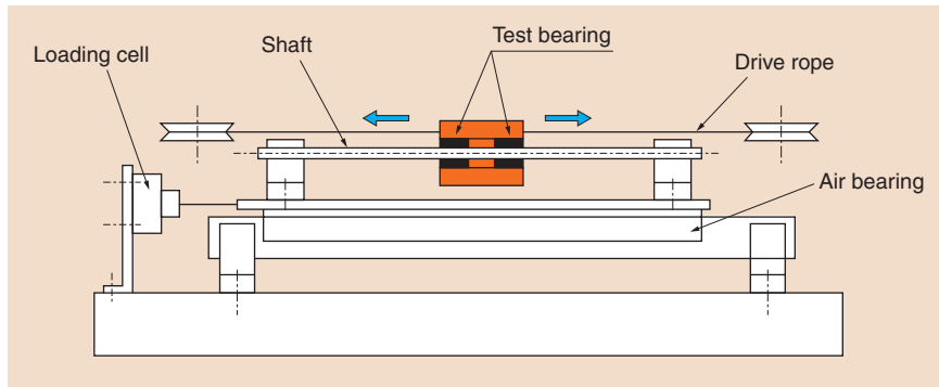
Fig. 6 Test Machine
