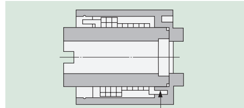
Rotating the NTS 18D in the direction opposite of the generated torque will cause locking tension to be concentrated on the hook section of the coil spring, leading to damage.
