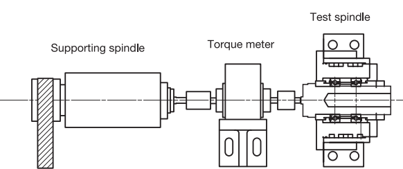
Test Bench Structure
