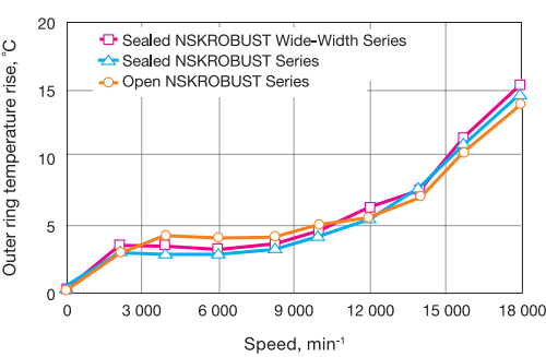
Comparison of Temperature Rise in Open vs. Sealed Bearings
