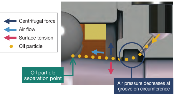
Structural Drawing of Spinshot™ II
