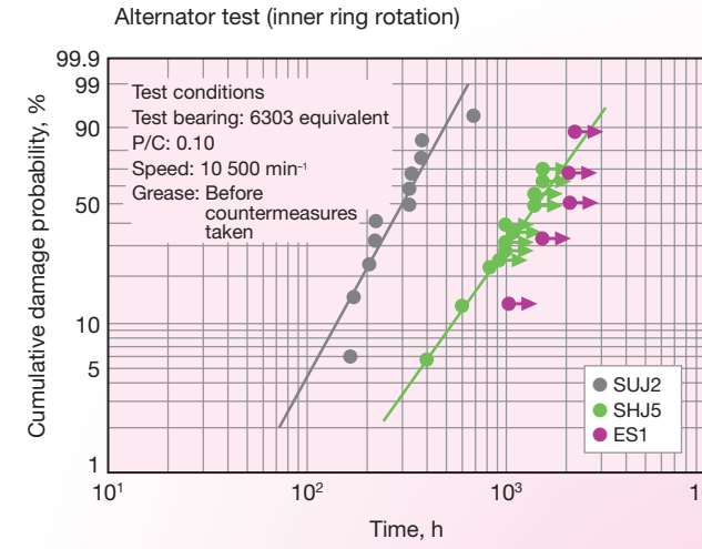
Results of white structure flaking durability test (material)
