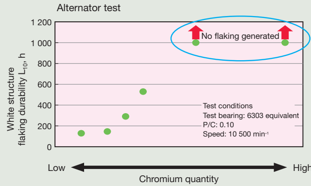
Relationship between chromium quantity and white structure flaking durability
