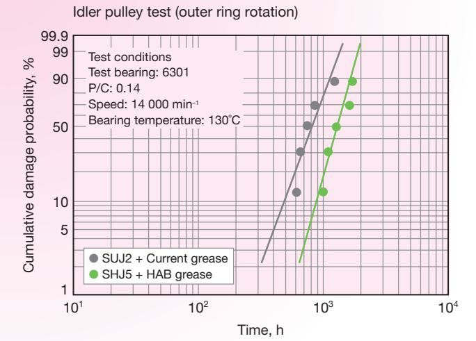
Results of seizure durability test (material)
