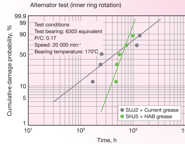
Results of seizure durability test (material)
