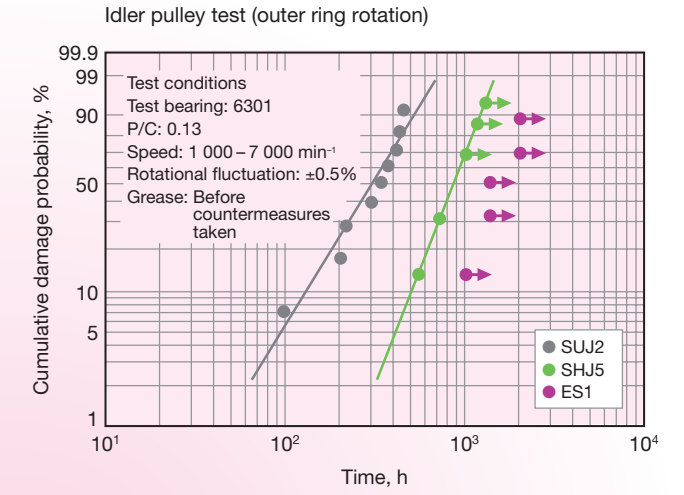
Results of white structure flaking durability test (material)
