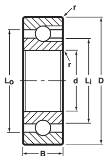
Unflanged
