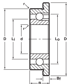
Flanged
