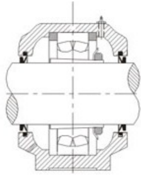
TA Type Design V-Ring with Lip Washer
