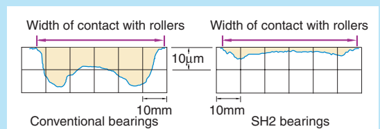
Fig. 7 Comparison between Conventional Bearings and SH2 Bearings in Wear (Inner ring raceway surface after 1 600 hours' use)
