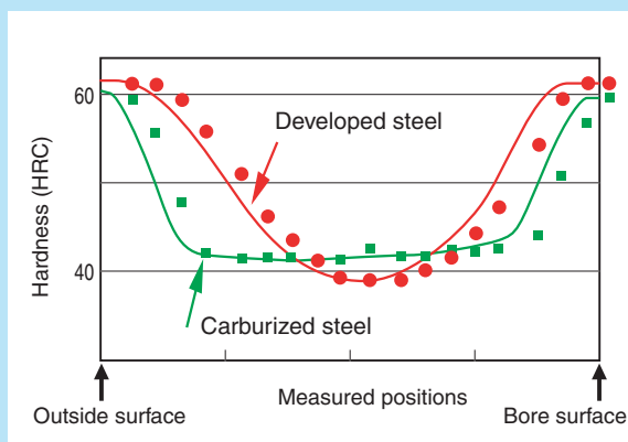
Fig. 3 Typical Hardness Distribution of cored hardening Outer Ring
