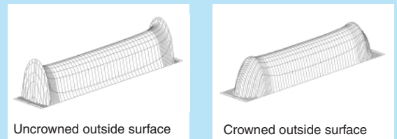
Fig. 5 Typical Contact Stress Distribution of Outer-ring Outside Surface
