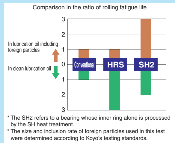
Fig. 6 Comparison of Long-life Materials in Service Life
