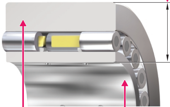
Fig. 2 Bearing Construction
