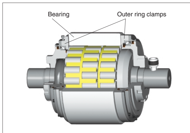
Fig. 10 Typical Installation of Suitable Bearing on Jig Type 2
