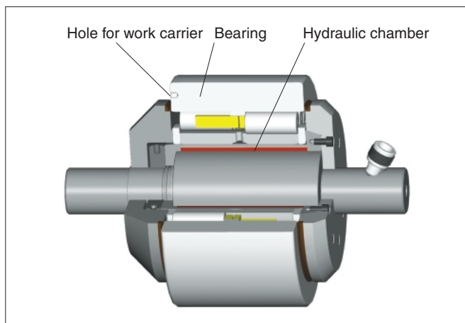
Fig. 9 Typical Installation of Suitable Bearing on Jig Type 1
