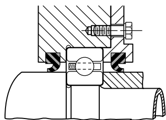
Figure 2-7 Nitrile Lip-Type Seal
