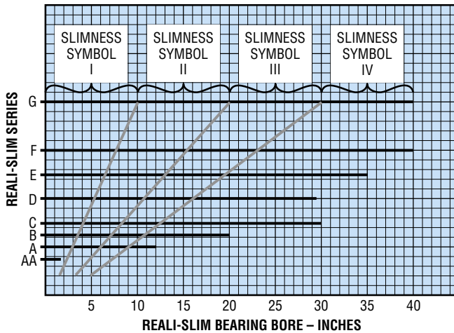
Figure 4-8 - Slimness Symbol (S 1 )
