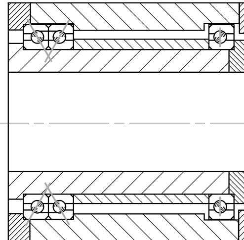
Figure 3-27B - Face to Face
