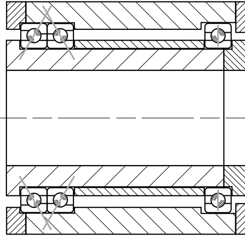
Figure 3-27A - Back to Back
