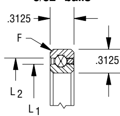
Snapover separator 5/32" balls
