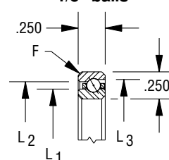
Circular pocket separator 1/8" balls
