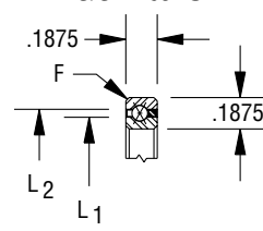
Snapover separator 3/32" balls
