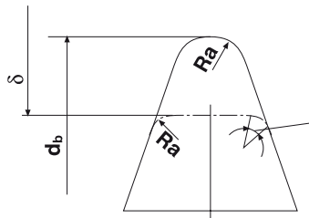
Detail Y: Groove top
