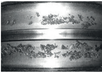
Figure 1 Fatigue spalling on the raceway
