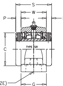
TWO BOLT
